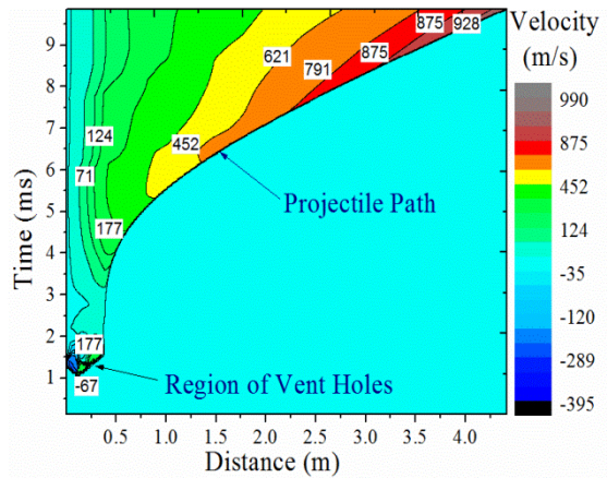
Fig.7. Gas phase velocity contours
