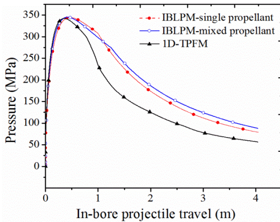
Fig.12. Pressure vs projectile displacement for different tools
