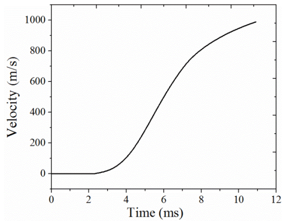
Fig.6. Projectile velocity curve for 1D-TPFM
