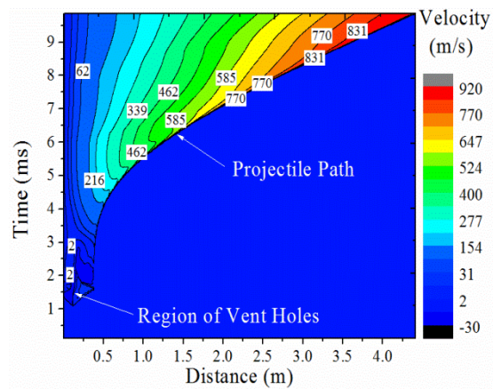
Fig.8. Solid phase velocity contours
