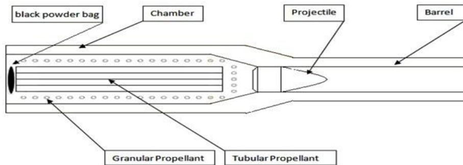
Fig.2. Gun system geometry with mixed propelling charge.
