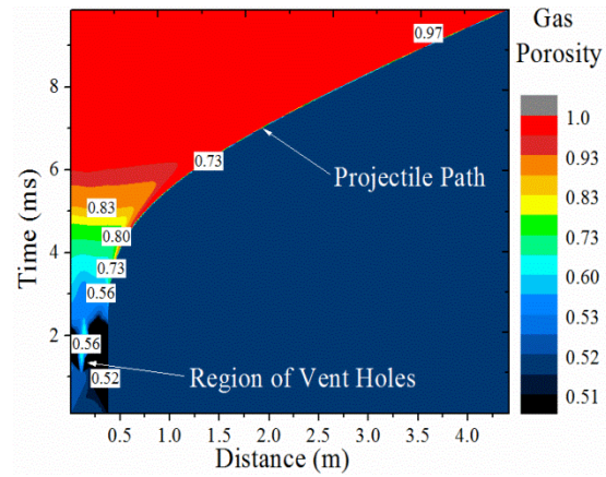
Fig.11. Gas phase volume fractions contours
