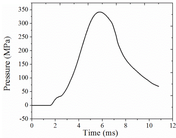
Fig.5. Pressure-vs-time curves for 1D-TPFM
