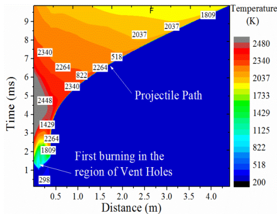
Fig.9. Gas phase temperature contours
