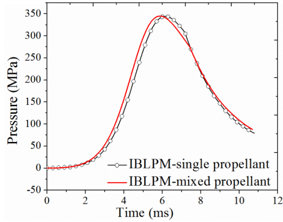
Fig.3. Pressure-vs-time curves for IBLPM
