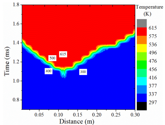
Fig.10. Solid phase temperature contours
