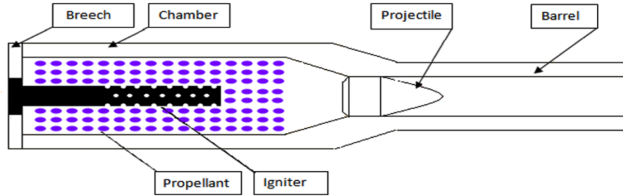
Fig.1. Gun system geometry with single propelling charge.
