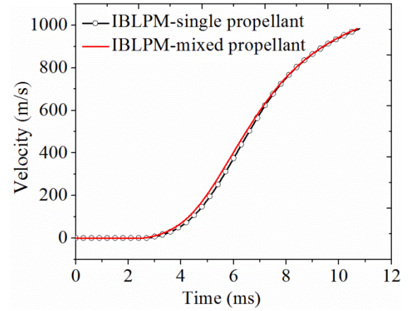
Fig.4. Projectile velocity curves for IBLPM
